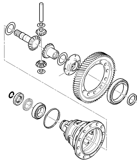
H Differential
