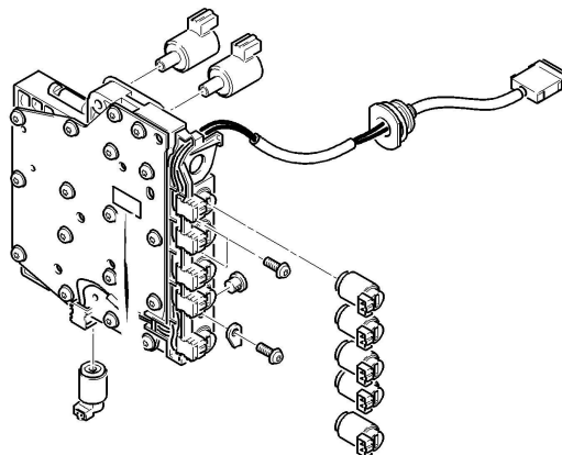
K Valvebody
