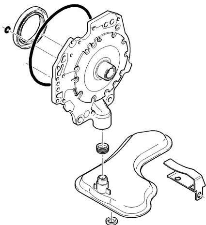
A Oilpump and Filter
