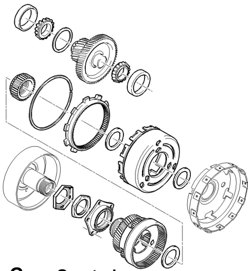
G Geartrain
